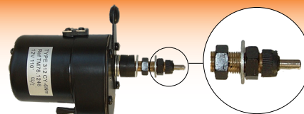
51045 Wiper Motor 12 Volt 110| Short Stem Straight Shaft Lenght 46mm Arm ref is 4296
