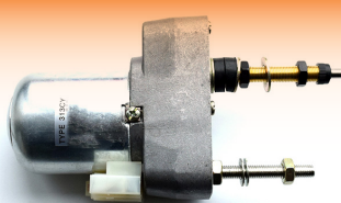
52956 Wiper Motor Case 40 43 44 45 56 95 12V OE Ref: 1535097C1
