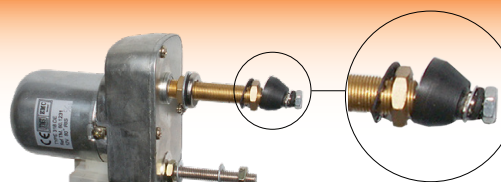
2492 Wiper Motor 12 Volt 110| Small Tapered Shaft Shaft Length 58mm
