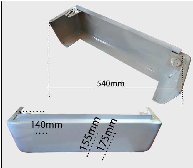
52648 Panel David Brown Lower 990 996 4 Cylinder
