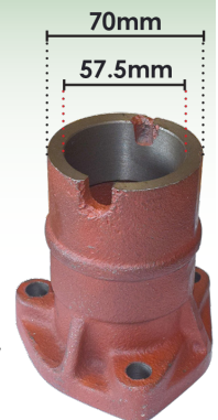
52178 Exhaust Manifold Elbow David Brown 1594 Also fits 1690 6 Cylinder
