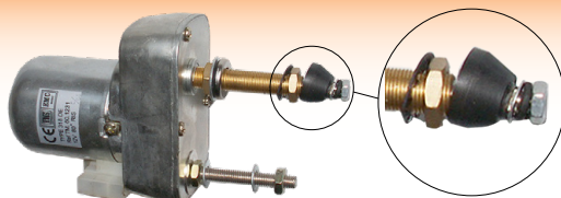
2491 Wiper Motor 12 Volt 80| Small Tapered Shaft Shaft Length 58mm - Check Type of Cab
