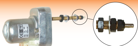
41656 Wiper Motor 12 Volt 120| Straight Single Spin Shaft Length 99mm
