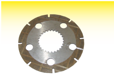
2333 Brake Disc David Brown 1490 Bronze 26 Splines 178mm (7")
