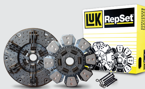
62100 Clutch Kit Valtra Mega 8300 8600 8800 12" Dual Disc 23 Splines 310/310mm OE Ref: 3580944M92
