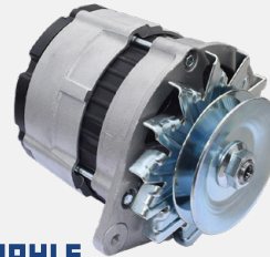
MAHLE Letrika 52479 Alternator 65 AMP Valtra 6000 Series 8000 Series OE Ref: K302424
