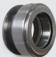
53784 A 700 900 800 600 500 300 400 200 Series OE Ref: V582990 ID 55mm OD 92.4mm Height 50mm
