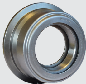
64537 PTO RELEASE BEARING Valtra Valmet 500 502 565 700 ID 70mm OD 133mm Width 58.31mm OE Ref: 654310
