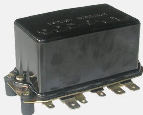
41620 Voltage Regulator Valtra / Valmet 502 565 361 22amp OE Ref: 81824174
