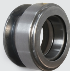
53784 CLUTCH RELEASE BEARING A 700 900 600 800 500 300 400 200 Series OE Ref: V582990 ID 55mm OD 92.4mm Height 50mm
